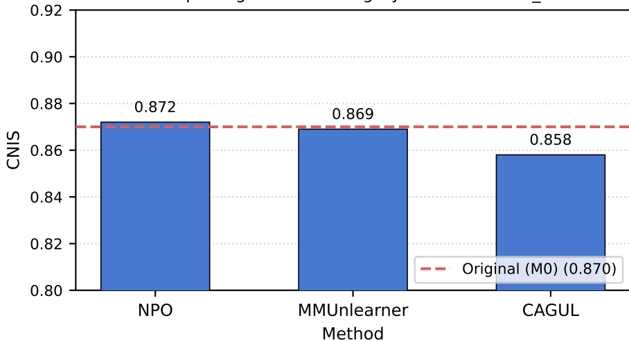
Concept Neighborhood Integrity Score — mllmu_real
