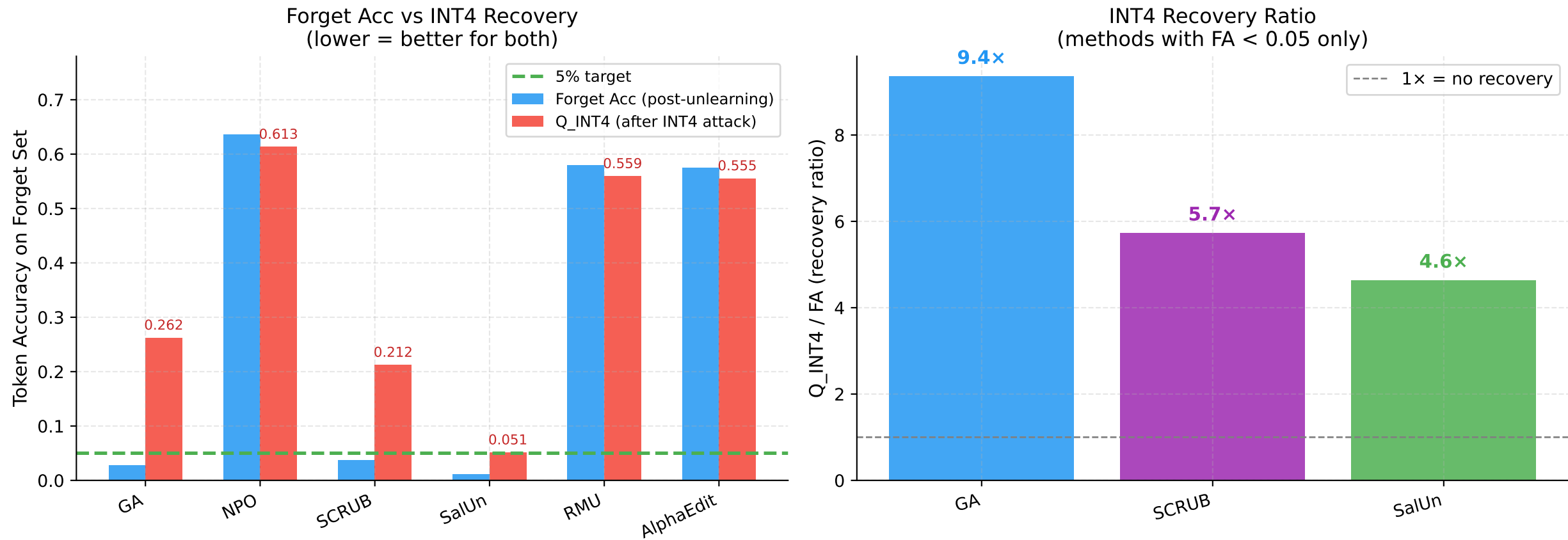
Figure 1: All 6 Baselines Fail Under INT4 Quantization Recovery Attack
