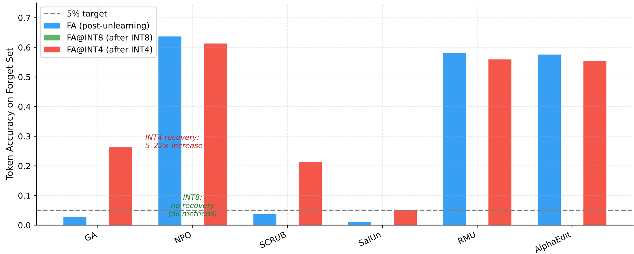
Figure 2: INT8 Quantization Is Harmless — INT4 Is a Universal Threat Q_INT8 = 0.000 for every method; Q_INT4 >> 0 for every method
