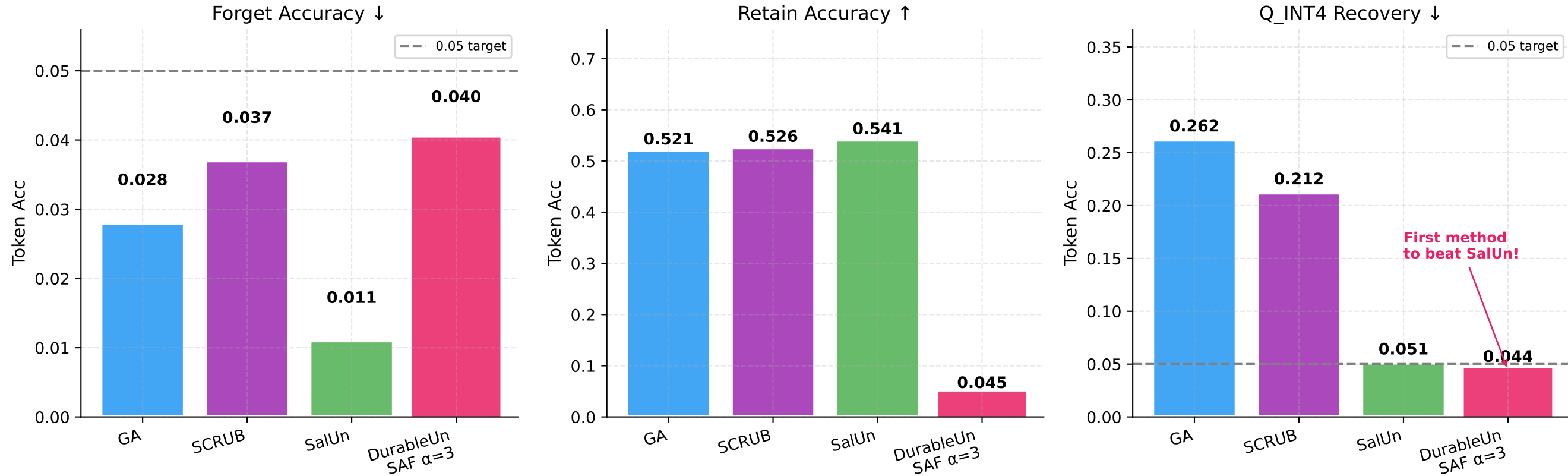
Figure 5: DurableUn-SAF vs Best Baselines (methods achieving FA < 0.05; DurableUn is first to beat SalUn Q_INT4)
