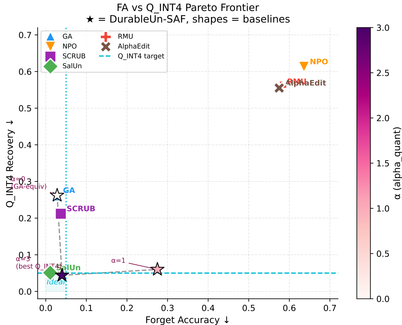
Figure 3: The FA-RA-Q_INT4 Trilemma — DurableUn-SAF Pareto Frontier
