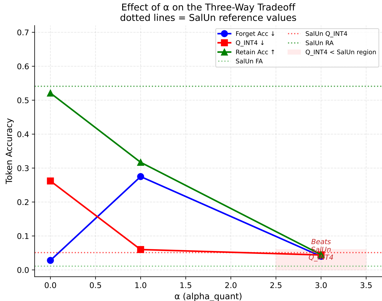
Figure 3: The FA-RA-Q_INT4 Trilemma — DurableUn-SAF Pareto Frontier
