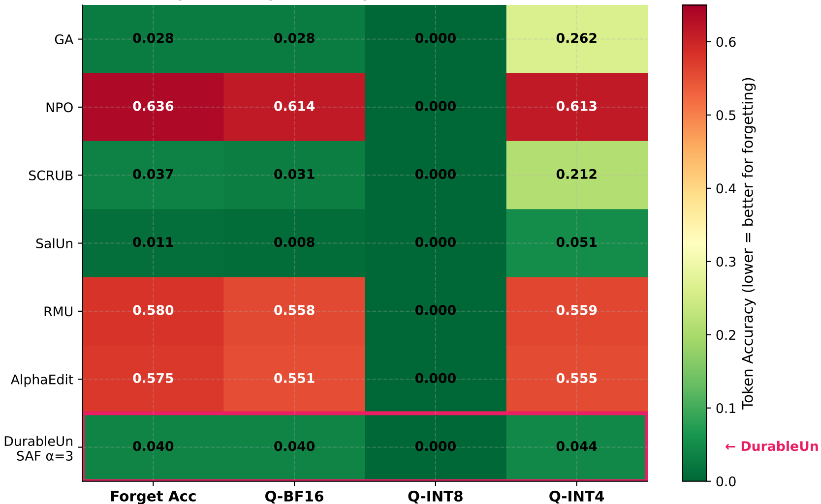
Figure 4: Forget Accuracy at Each Quantization Precision (green=low=good, red=high=model still remembers)
