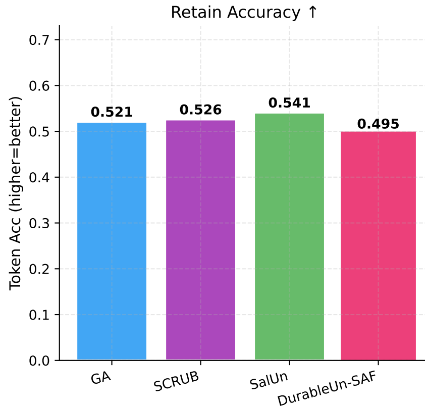
Figure 4: DurableUn-SAF vs Best Baselines (methods achieving FA < 0.05)
