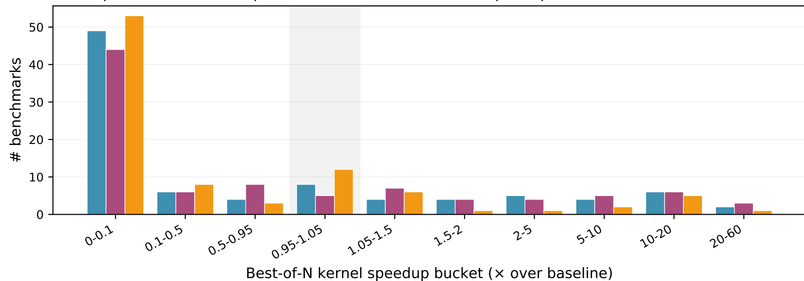
EX2 (OpenMP, 16 threads): per-benchmark best-of-N kernel speedup distribution
