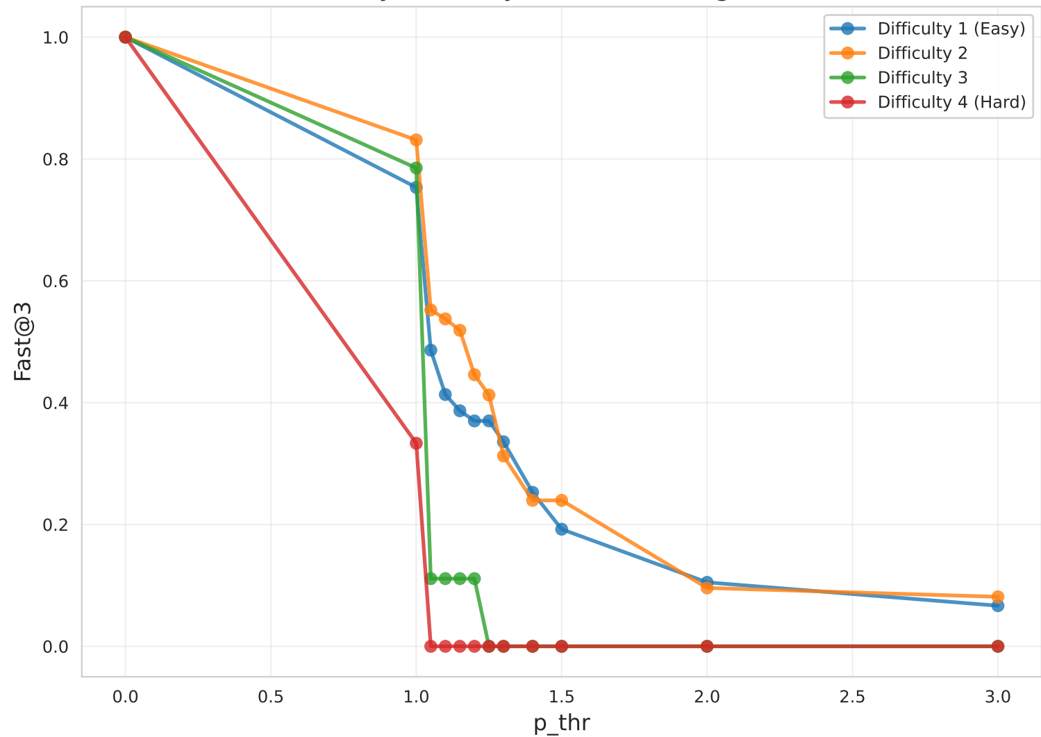
Fast@3 by Difficulty (EX1, extra-large, Claude)
