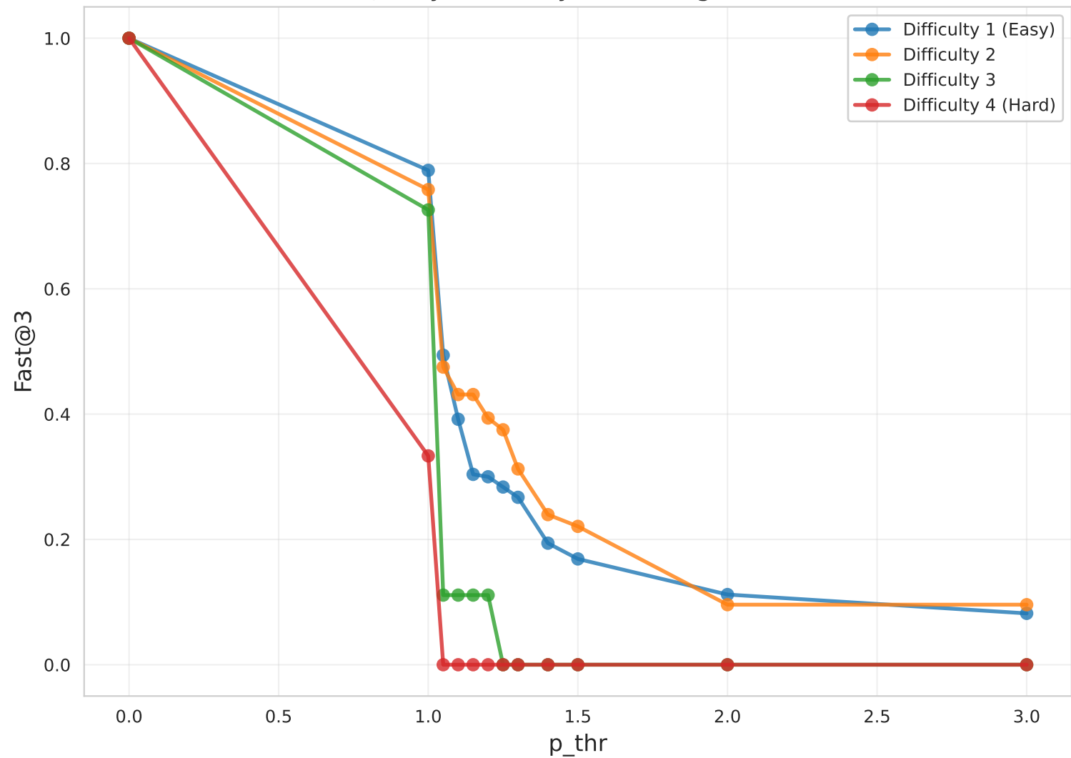
Fast@3 by Difficulty (EX1, large, Claude)
