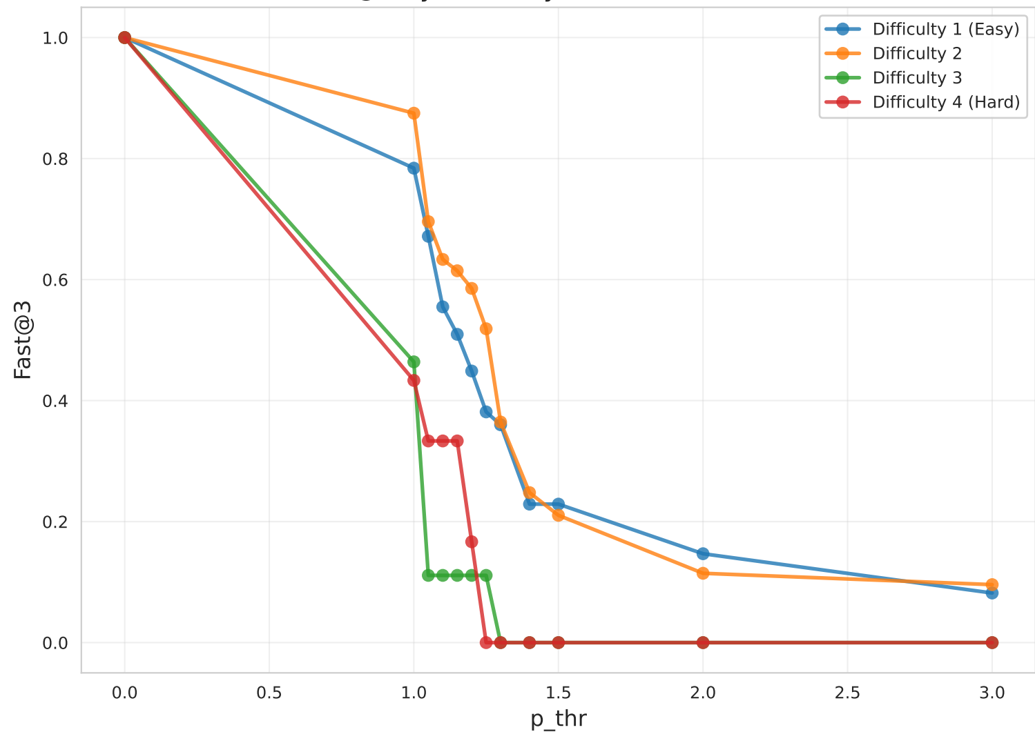
Fast@3 by Difficulty (EX1, mini, Claude)
