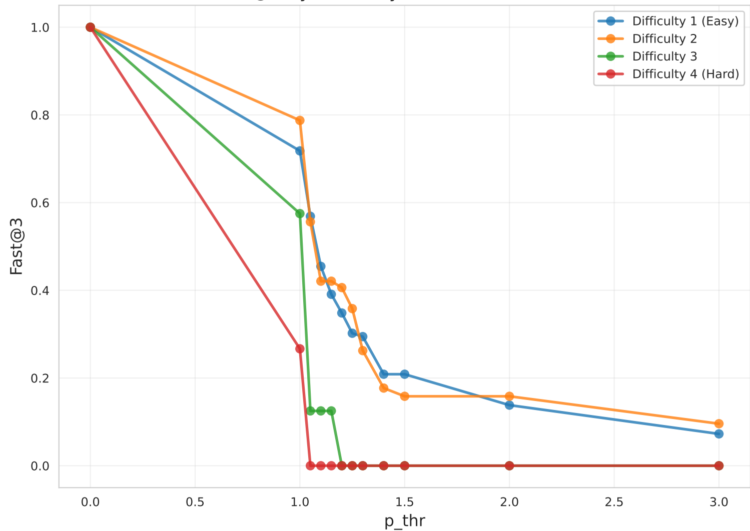
Fast@3 by Difficulty (EX1, small, Claude)
