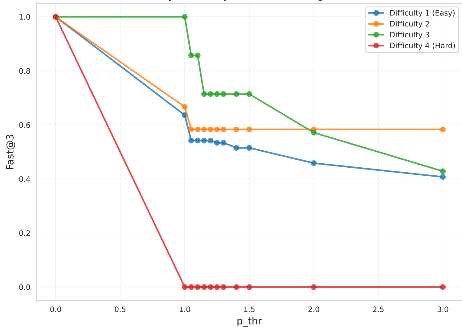
Fast@3 by Difficulty (EX2, extra-large, Claude)
