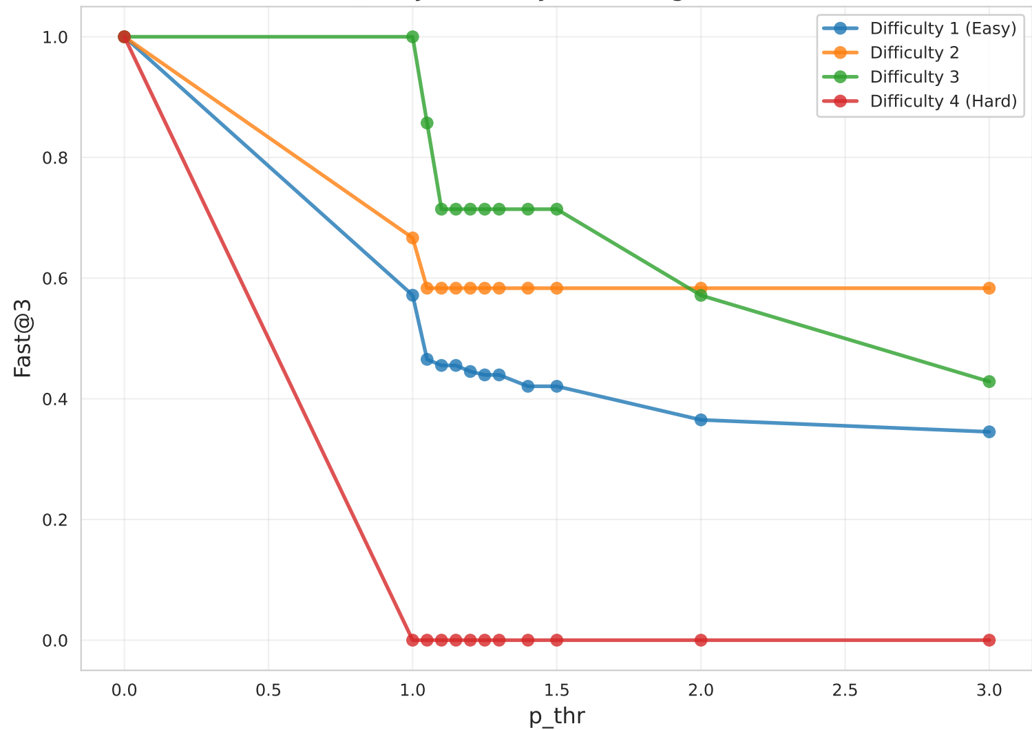
Fast@3 by Difficulty (EX2, large, Claude)
