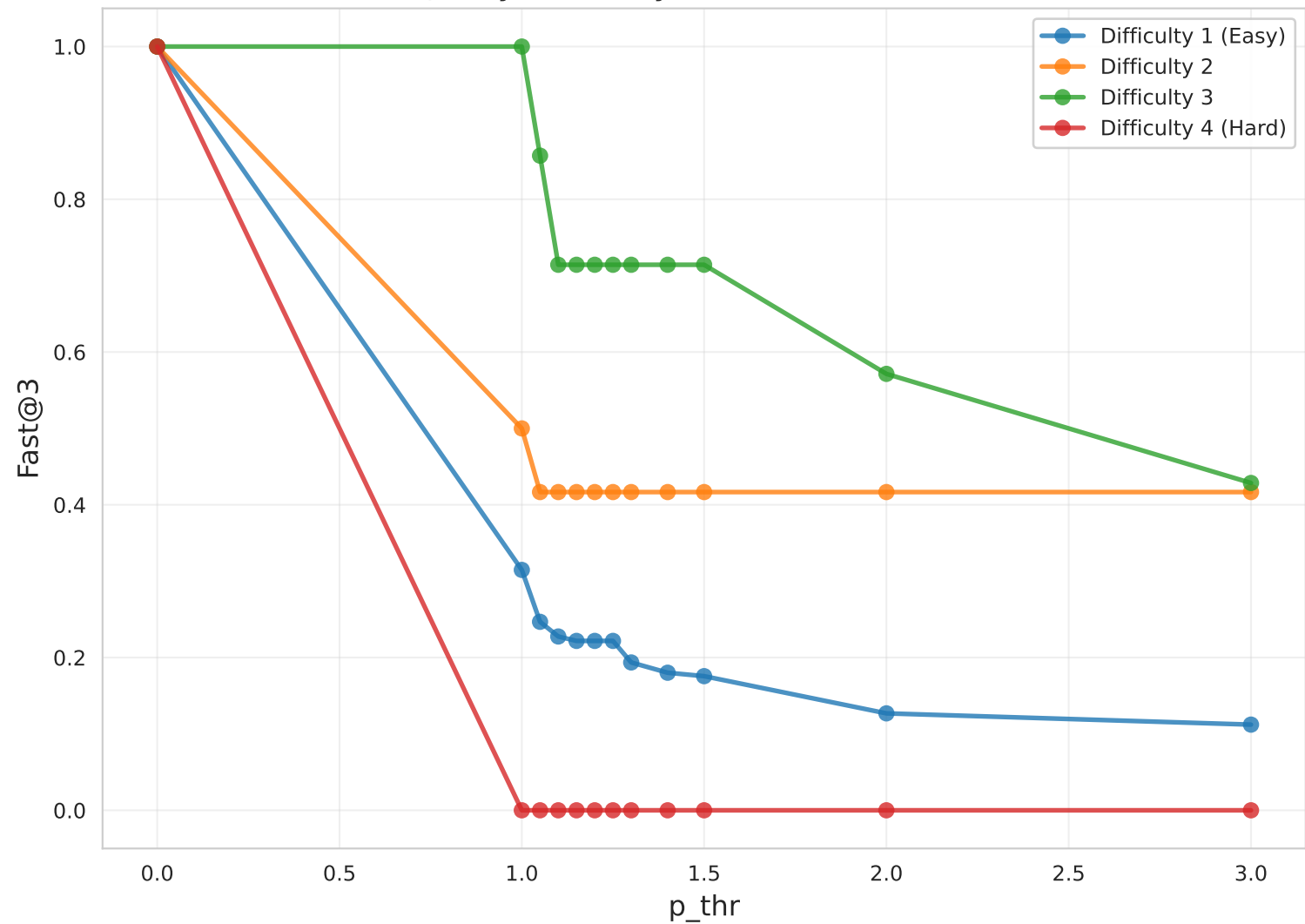
Fast@3 by Difficulty (EX2, medium, Claude)
