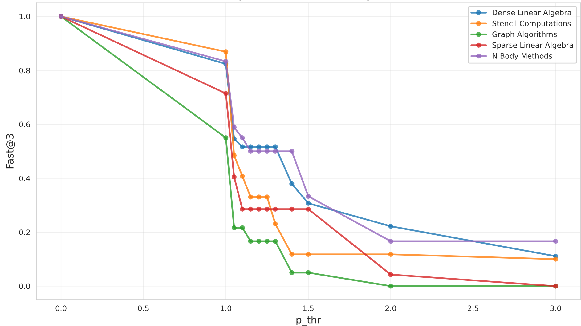
Fast@3 by Motif (EX1, extra-large, Claude)
