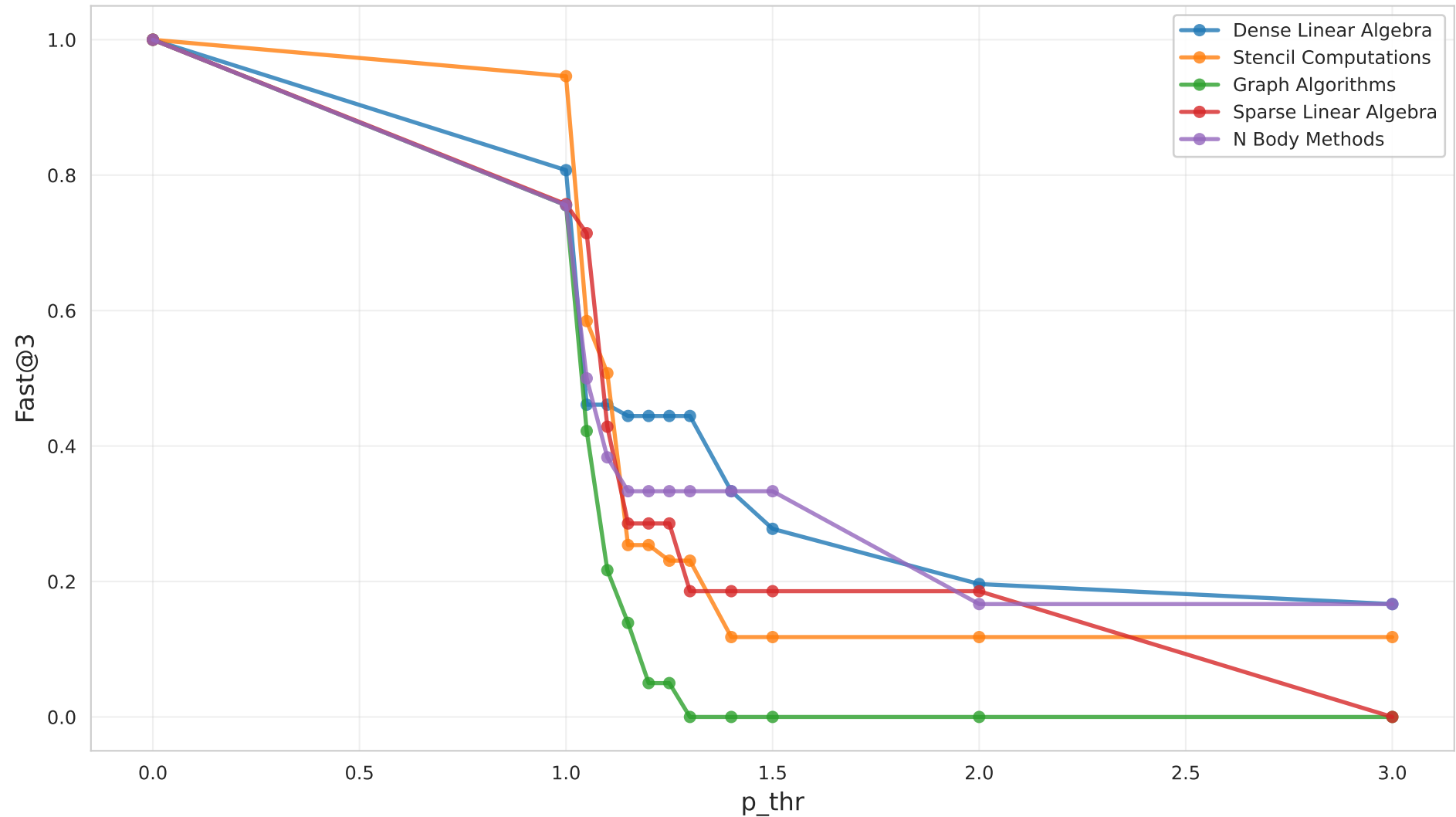
Fast@3 by Motif (EX1, large, Claude)
