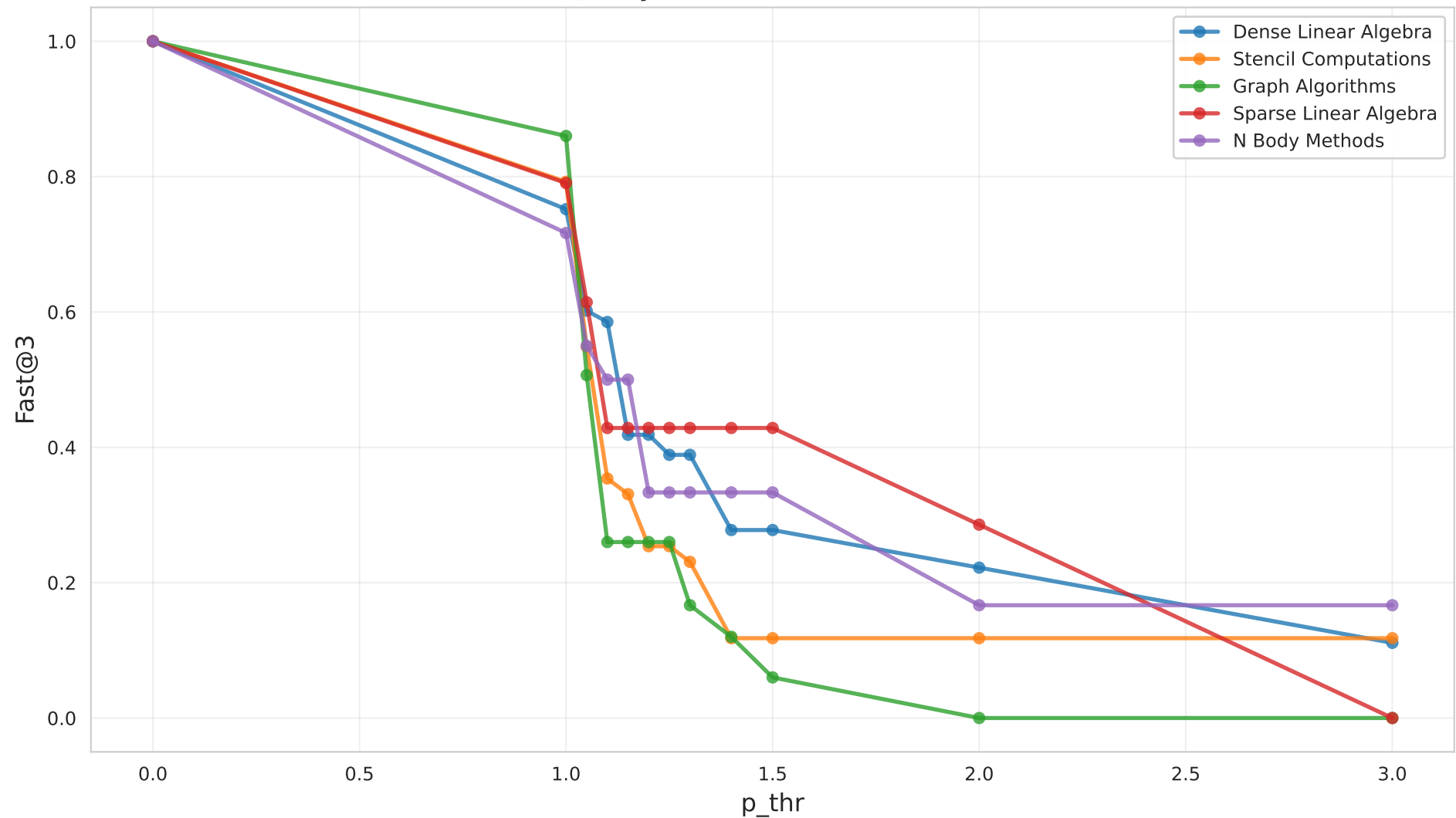
Fast@3 by Motif (EX1, small, Claude)
