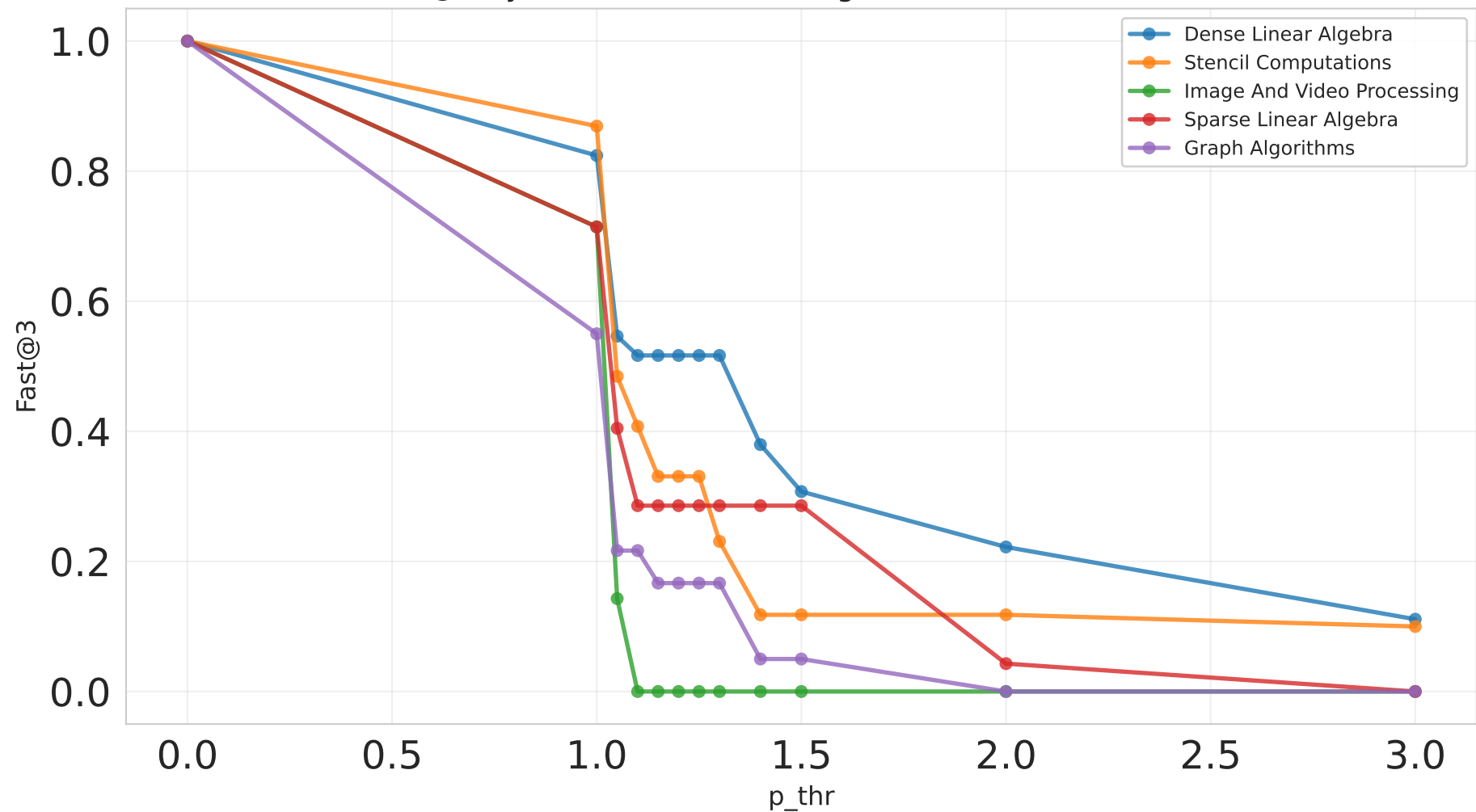
Fast@3 by Motif (EX1, extra-large, Claude, All Difficulties)
