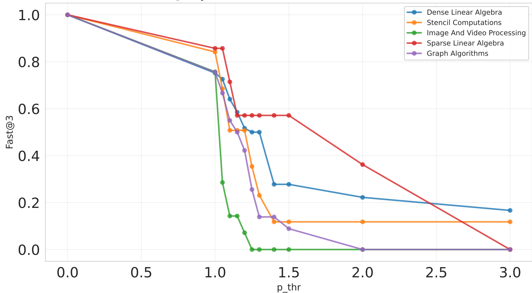
Fast@3 by Motif (EX1, mini, Claude, All Difficulties)
