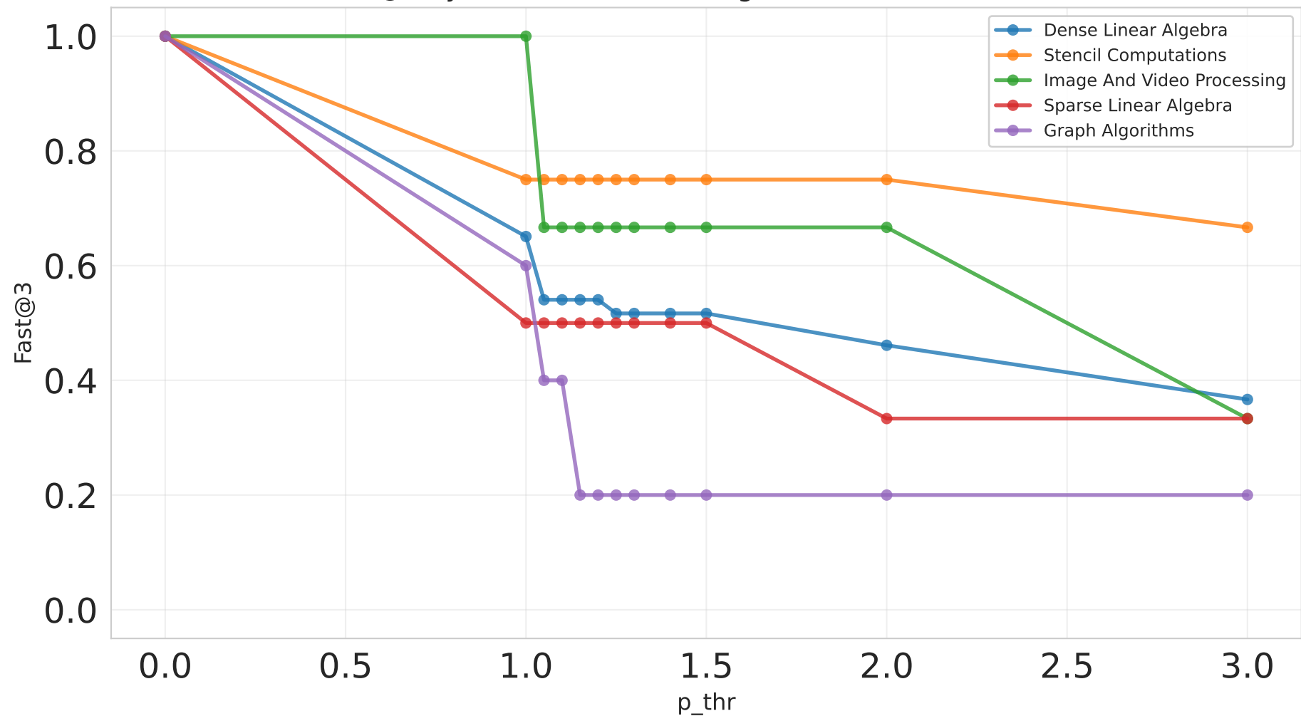
Fast@3 by Motif (EX2, extra-large, Claude, All Difficulties)
