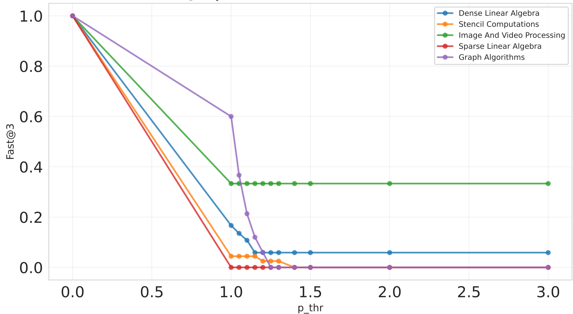
Fast@3 by Motif (EX2, mini, Claude, All Difficulties)
