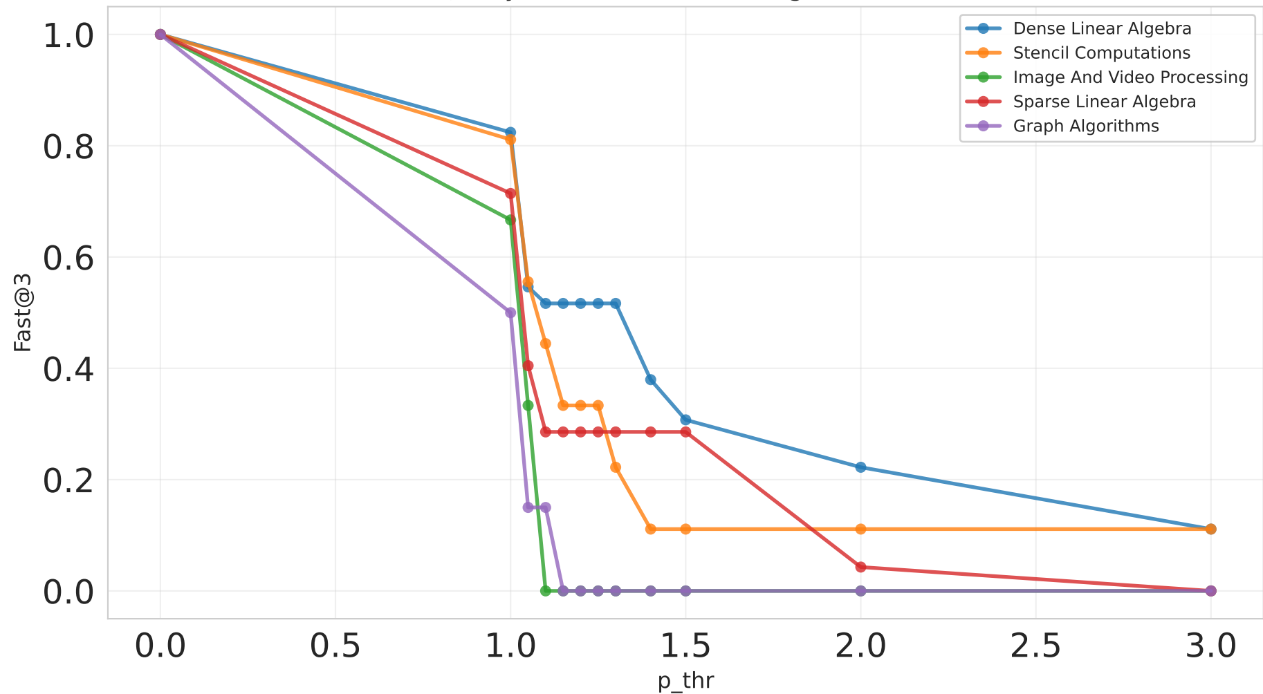
Fast@3 by Motif (EX1, extra-large, Claude, d1)
