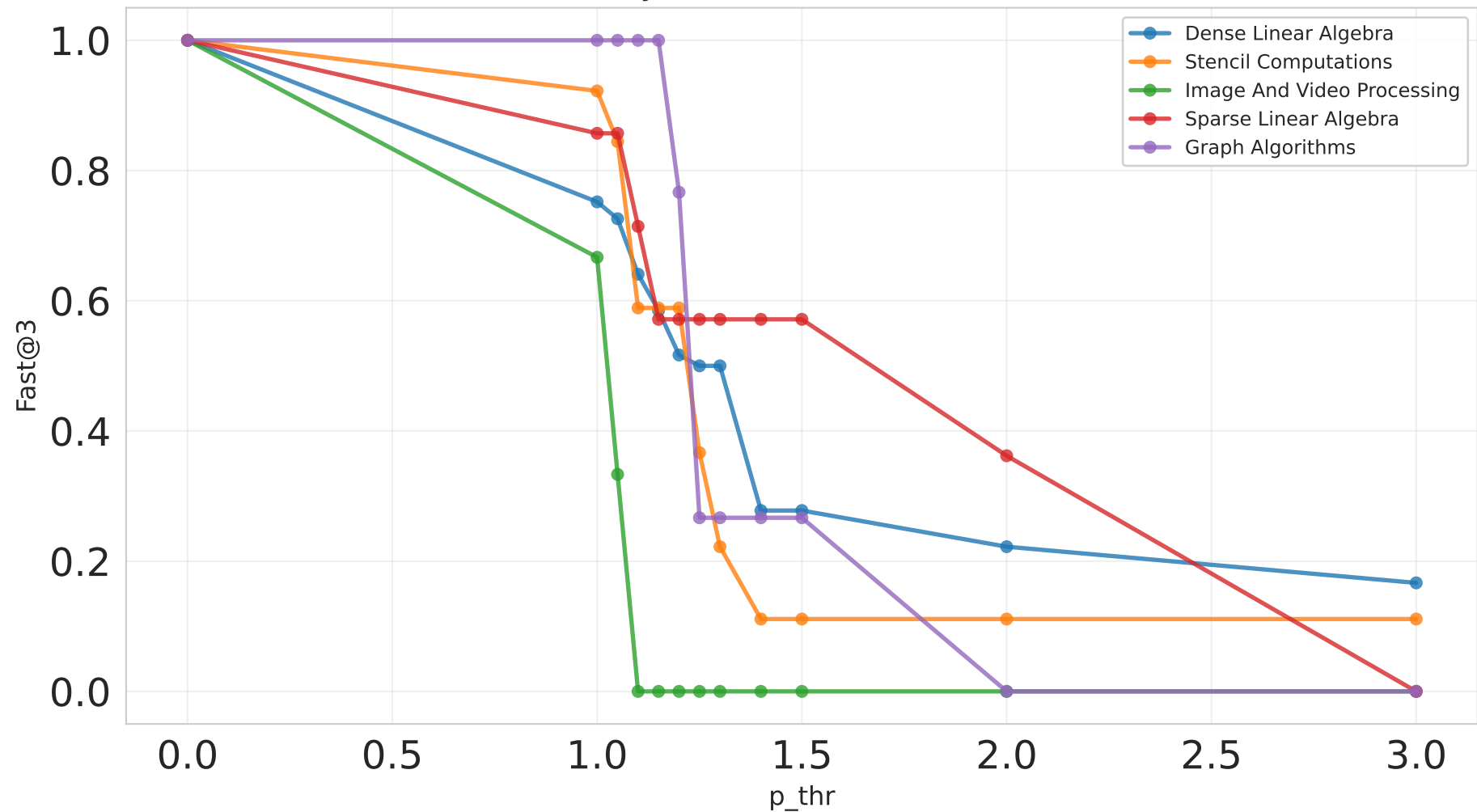
Fast@3 by Motif (EX1, mini, Claude, d1)
