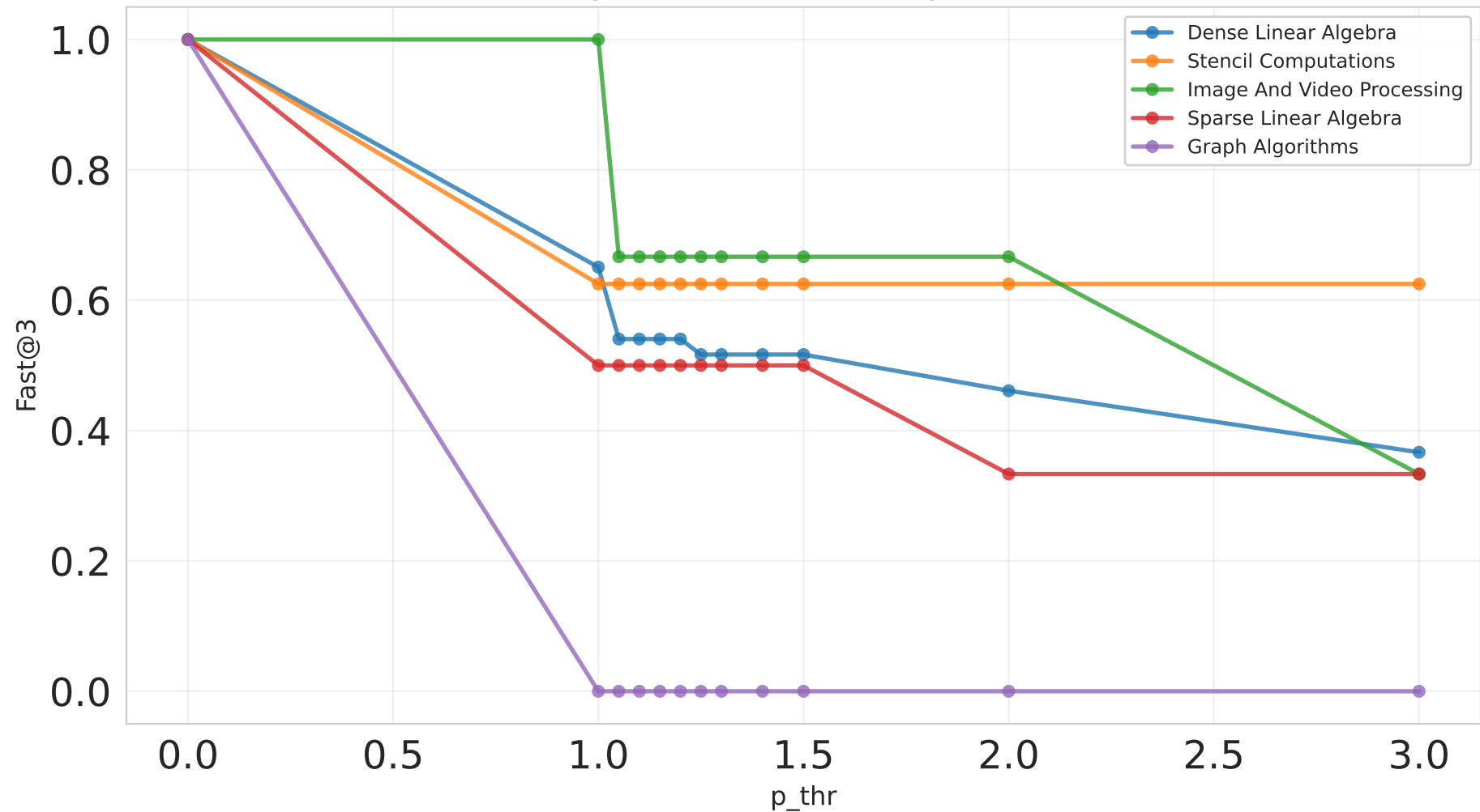
Fast@3 by Motif (EX2, extra-large, Claude, d1)
