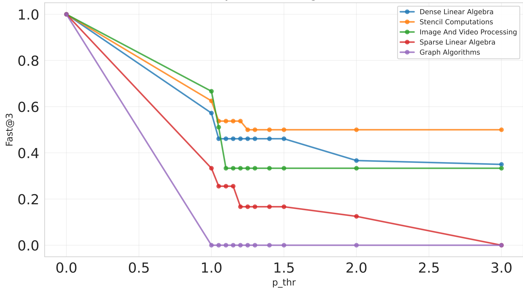
Fast@3 by Motif (EX2, large, Claude, d1)
