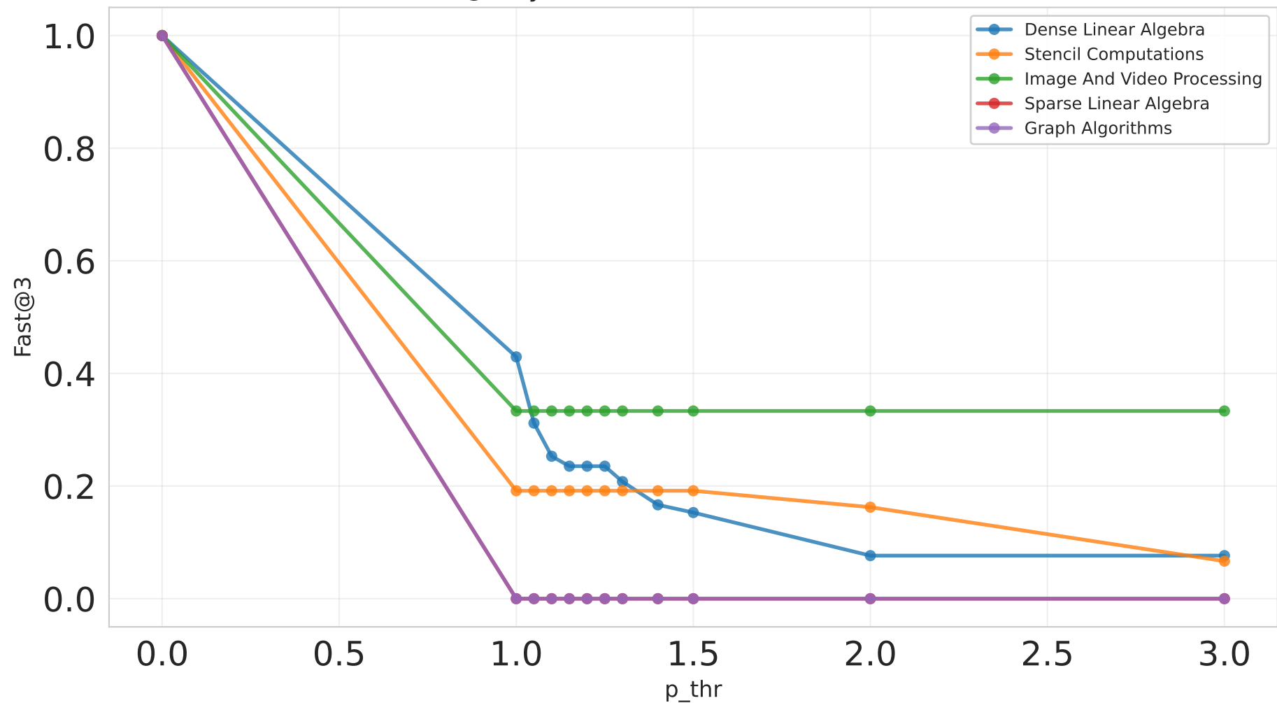
Fast@3 by Motif (EX2, medium, Claude, d1)
