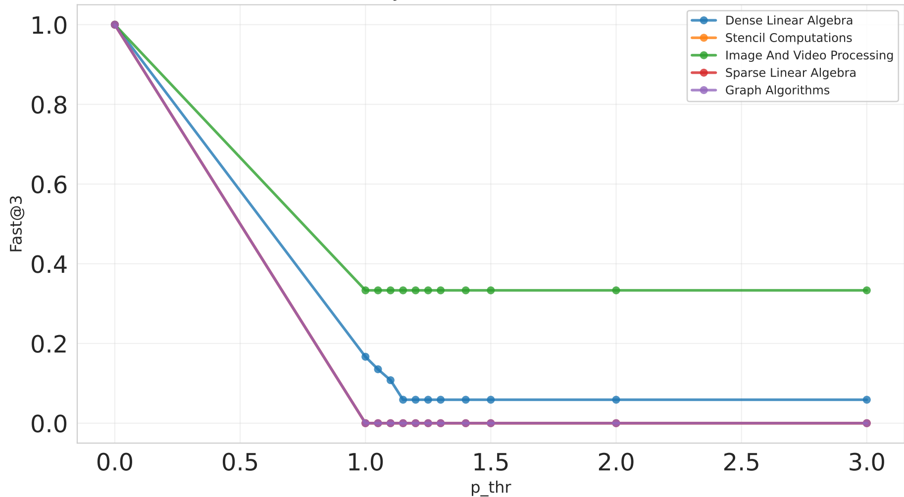
Fast@3 by Motif (EX2, mini, Claude, d1)
