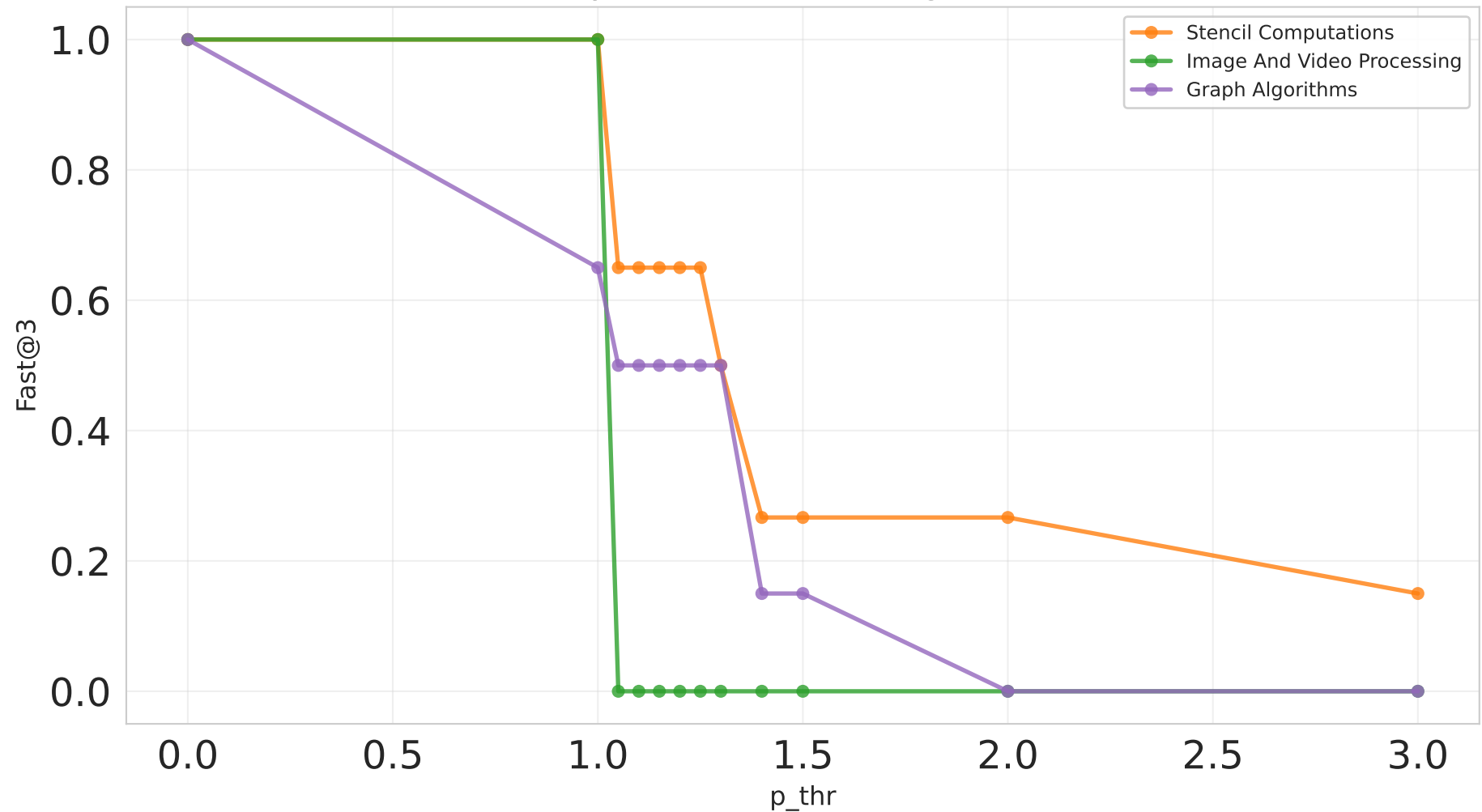
Fast@3 by Motif (EX1, extra-large, Claude, d2)
