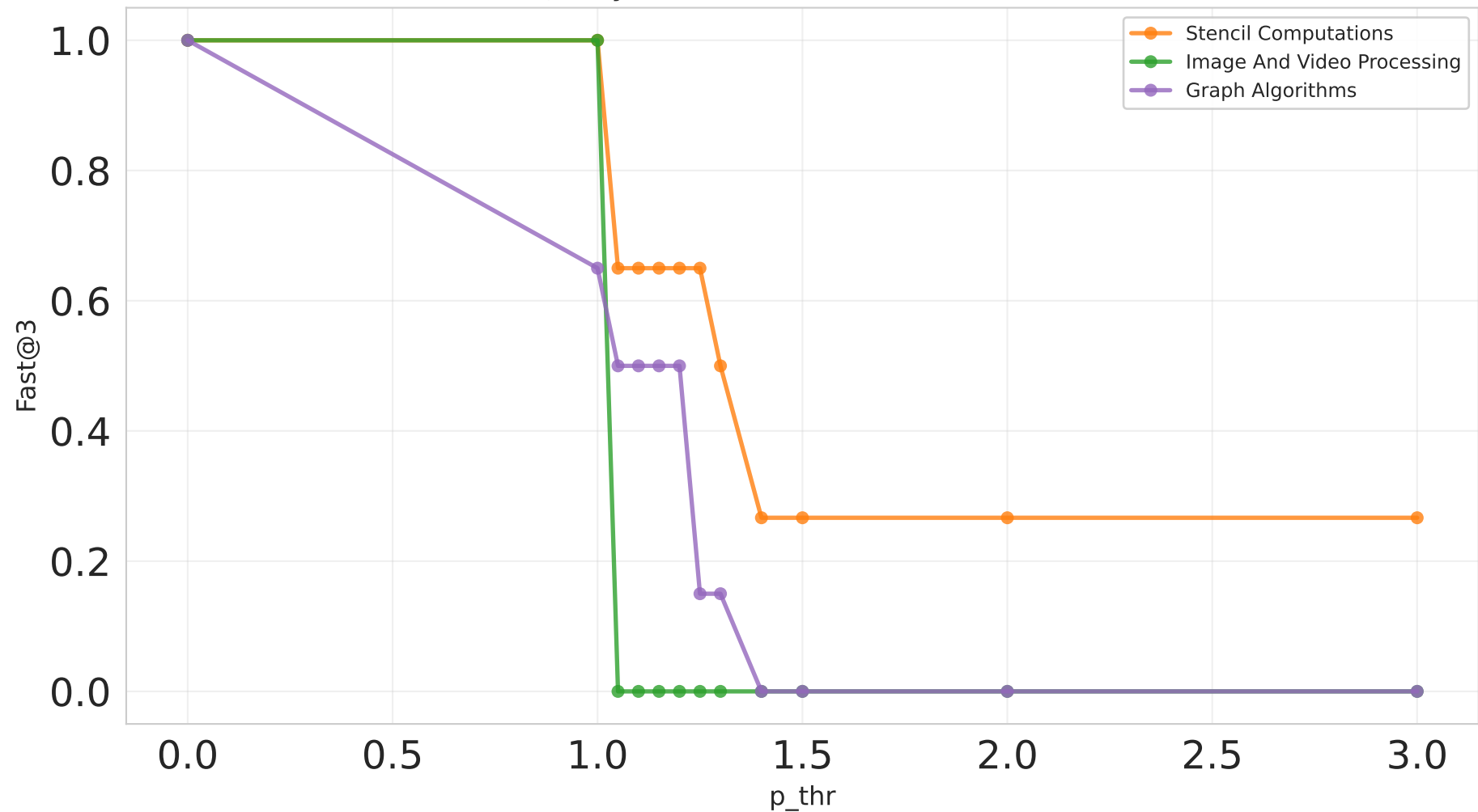
Fast@3 by Motif (EX1, medium, Claude, d2)
