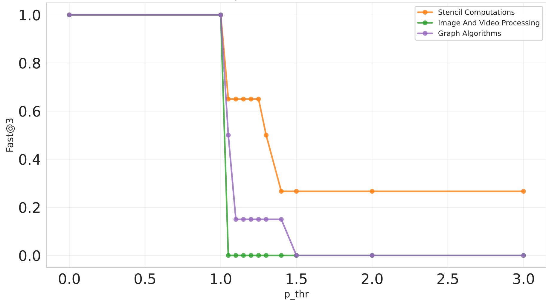
Fast@3 by Motif (EX1, small, Claude, d2)
