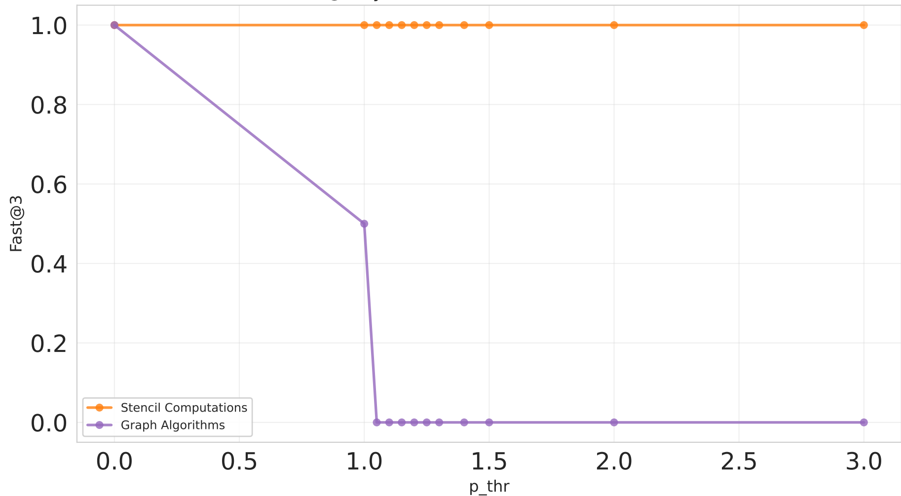
Fast@3 by Motif (EX2, medium, Claude, d2)
