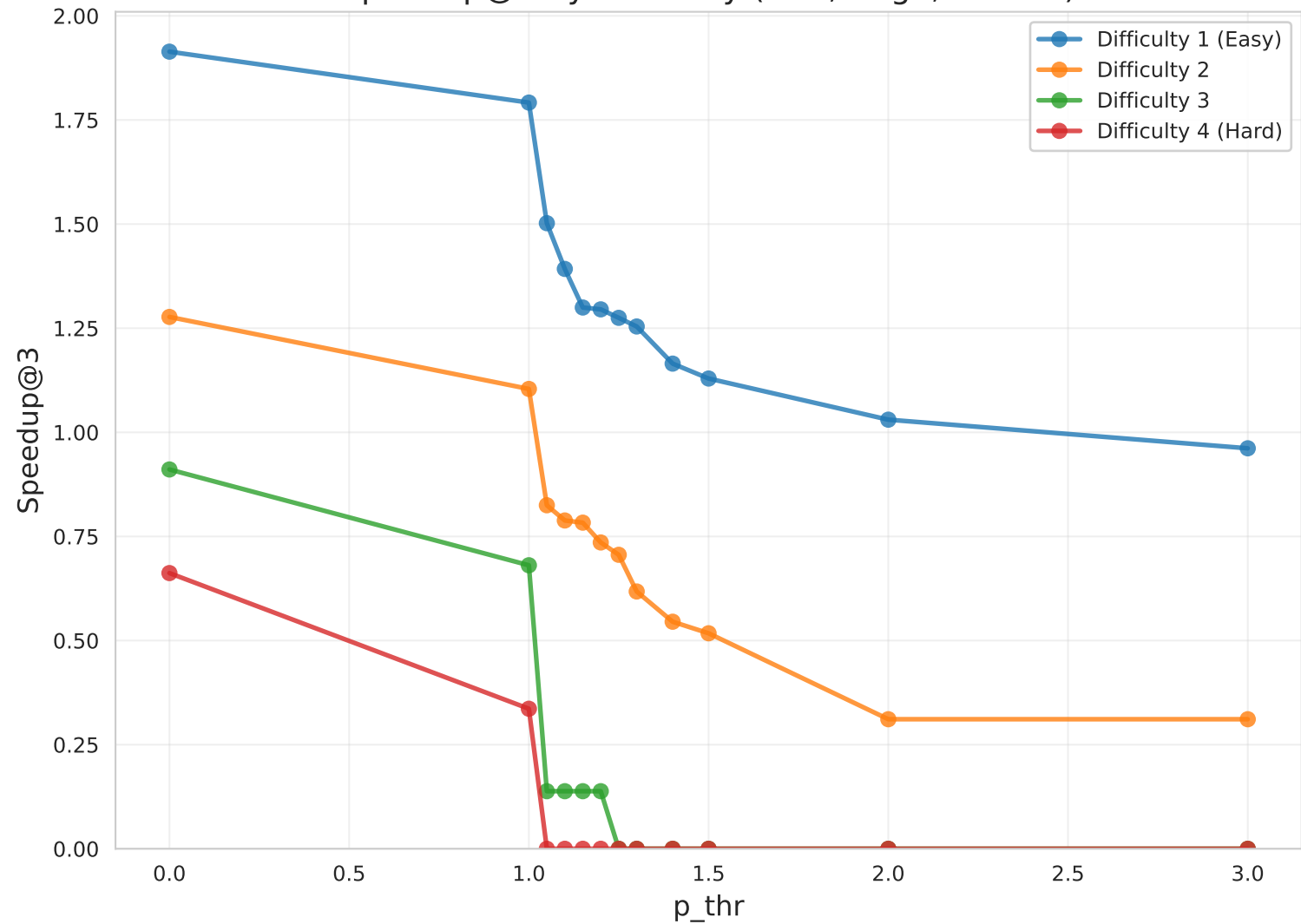
Speedup@3 by Difficulty (EX1, large, Claude)
