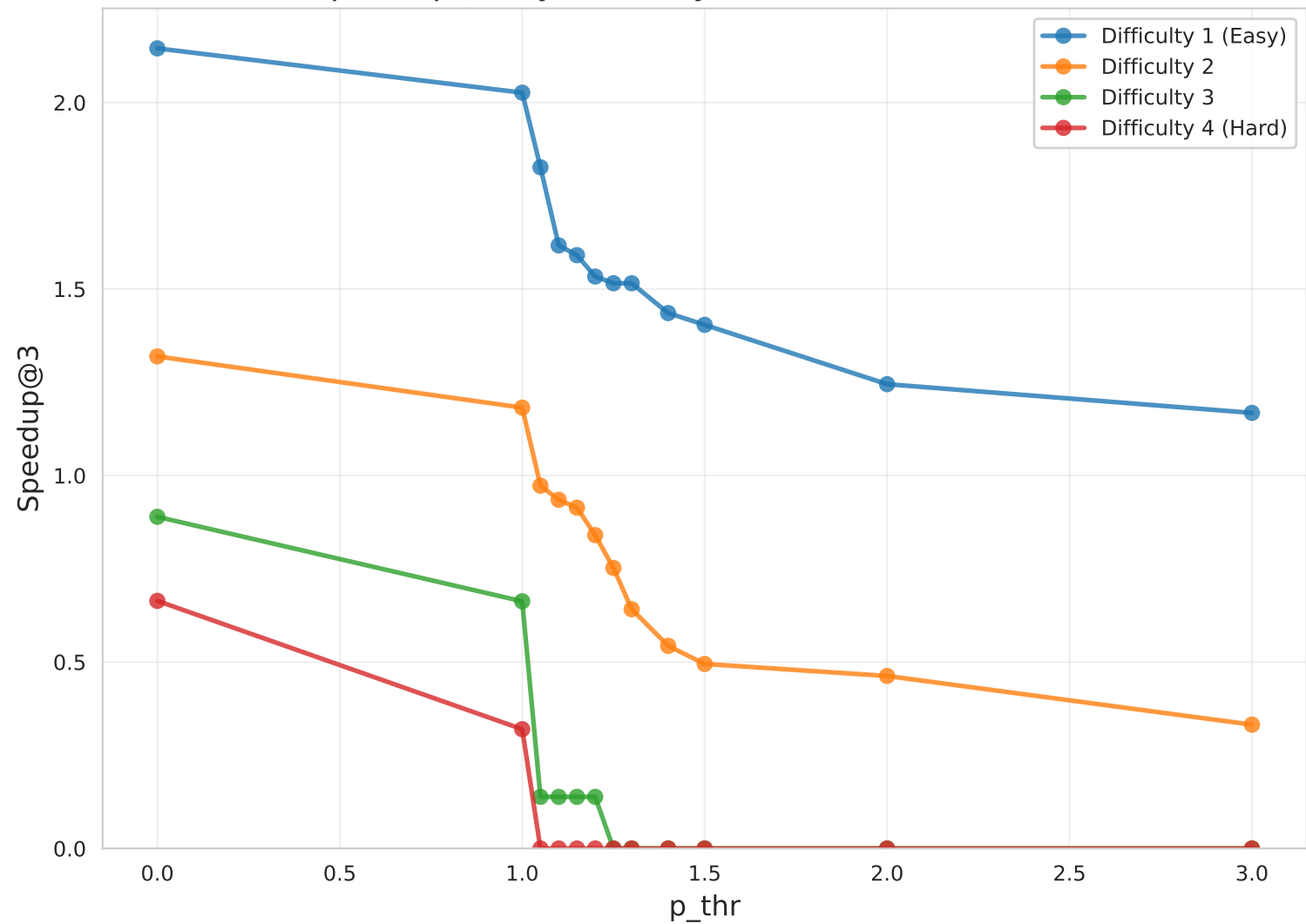
Speedup@3 by Difficulty (EX1, medium, Claude)
