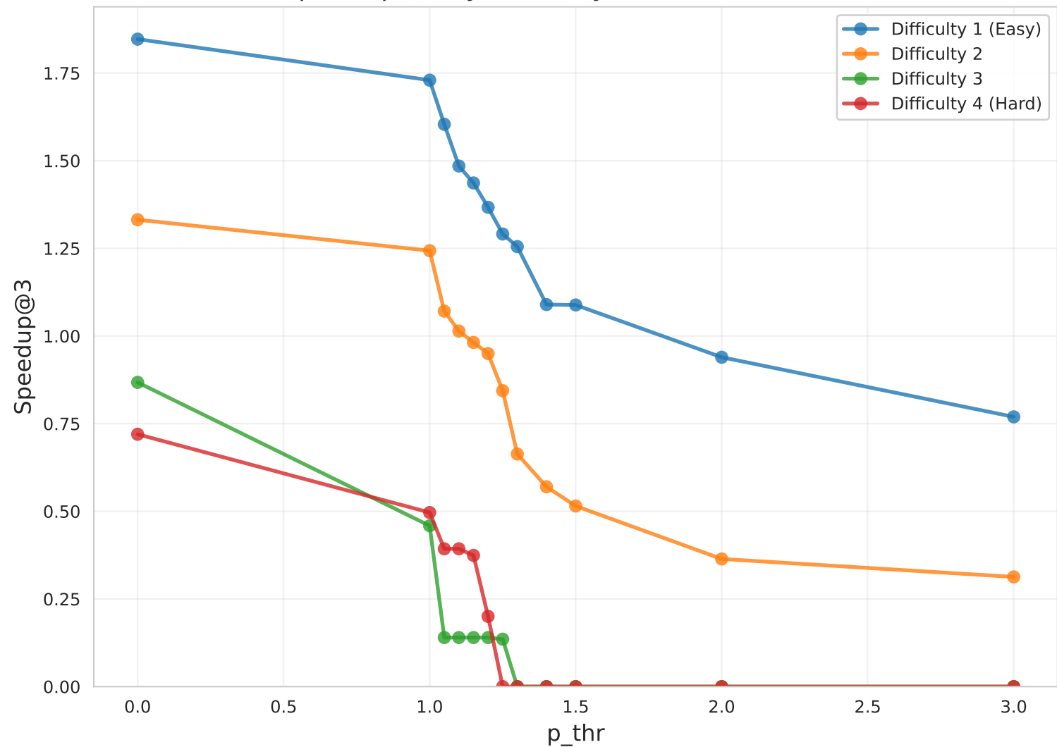
Speedup@3 by Difficulty (EX1, mini, Claude)
