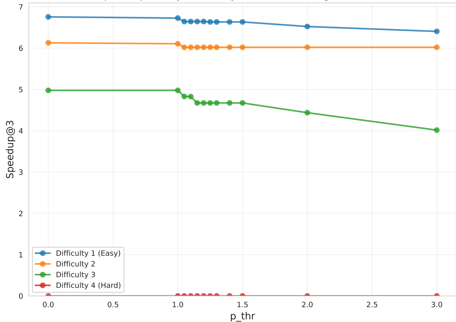
Speedup@3 by Difficulty (EX2, extra-large, Claude)
