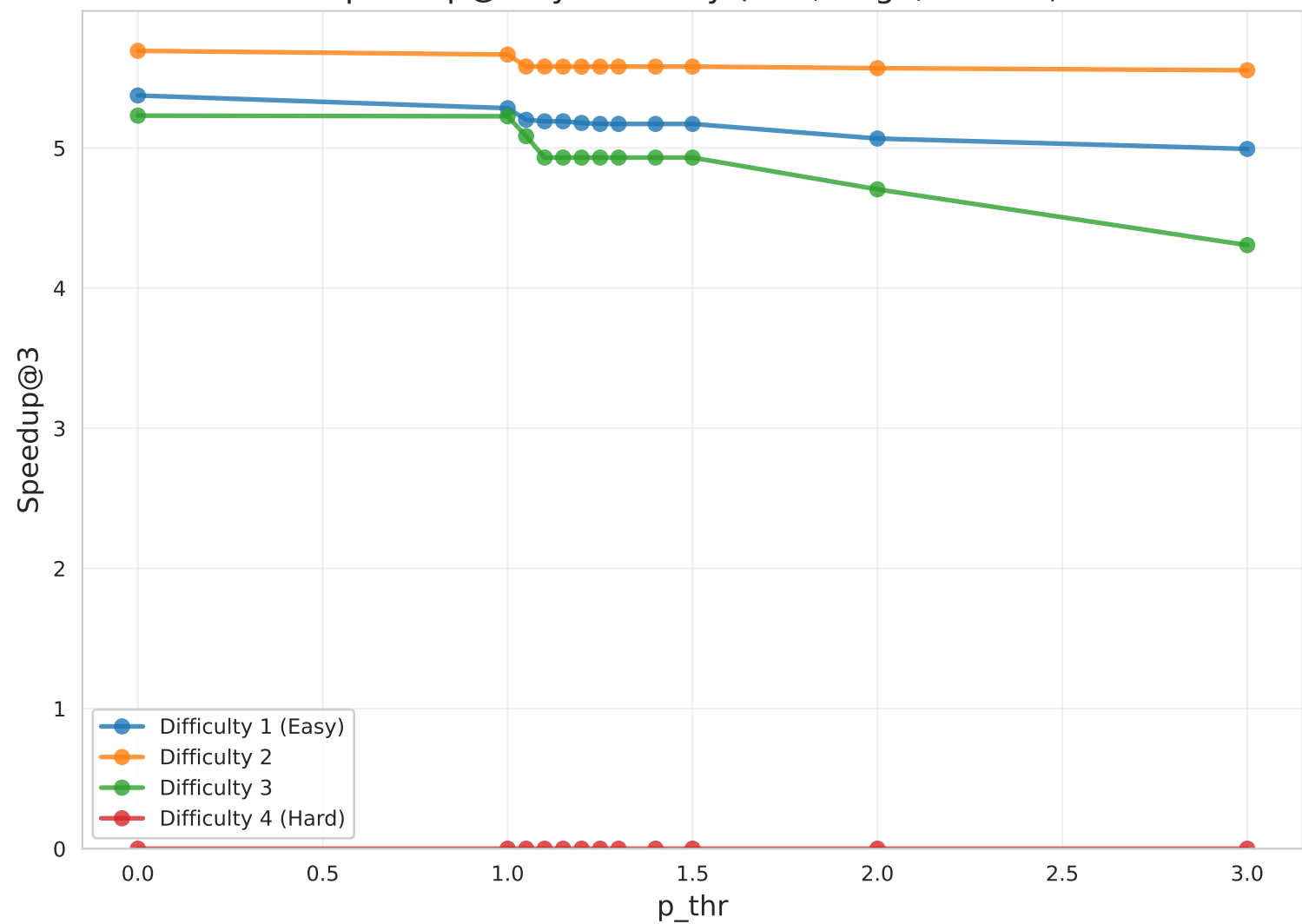
Speedup@3 by Difficulty (EX2, large, Claude)
