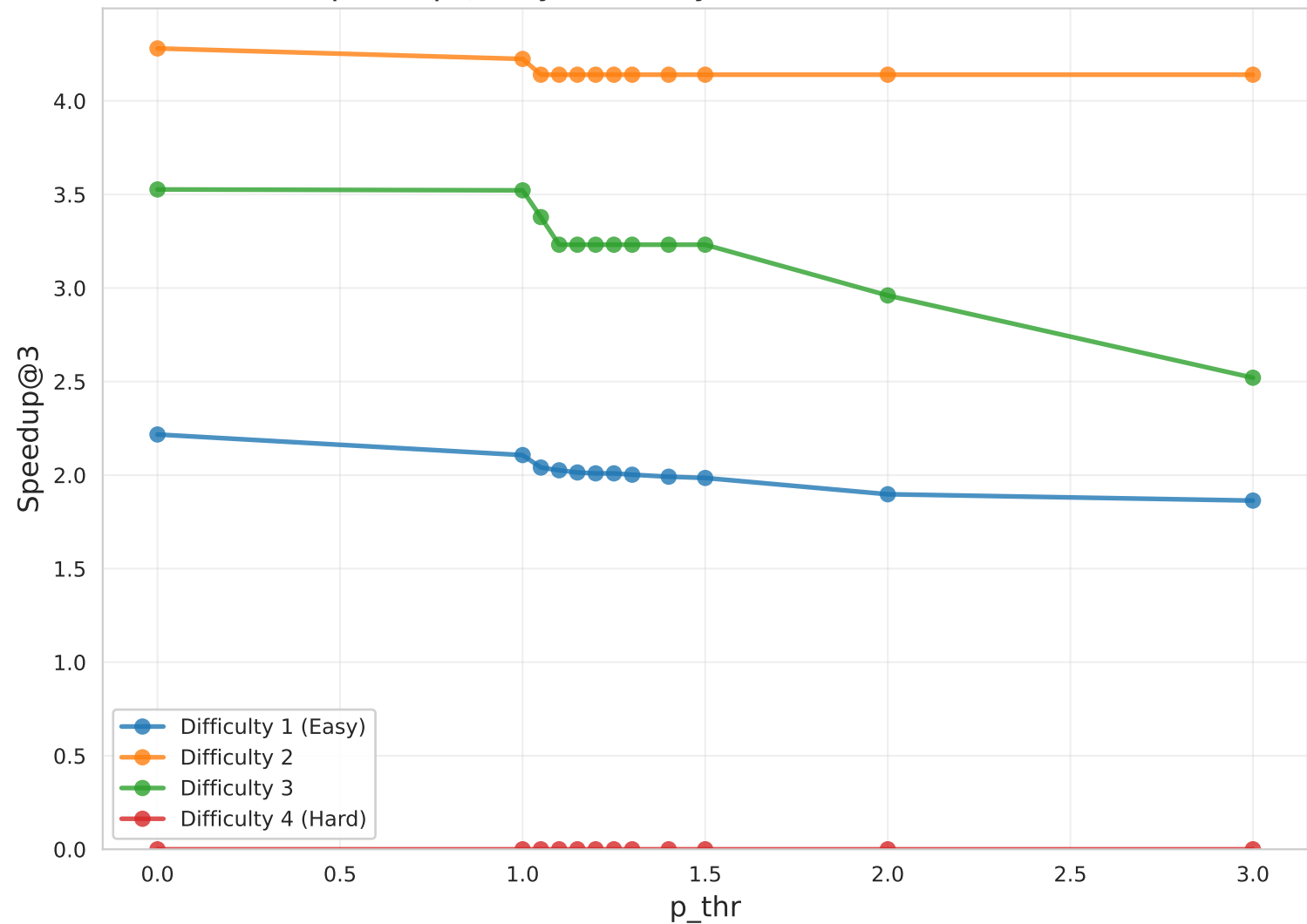
Speedup@3 by Difficulty (EX2, medium, Claude)
