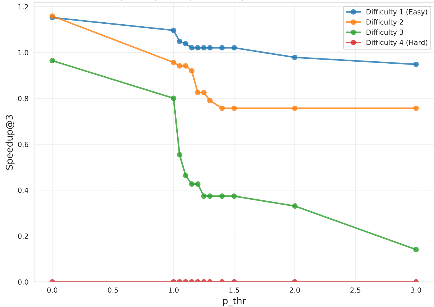
Speedup@3 by Difficulty (EX2, mini, Claude)
