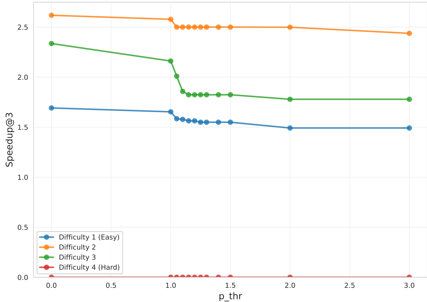
Speedup@3 by Difficulty (EX2, small, Claude)
