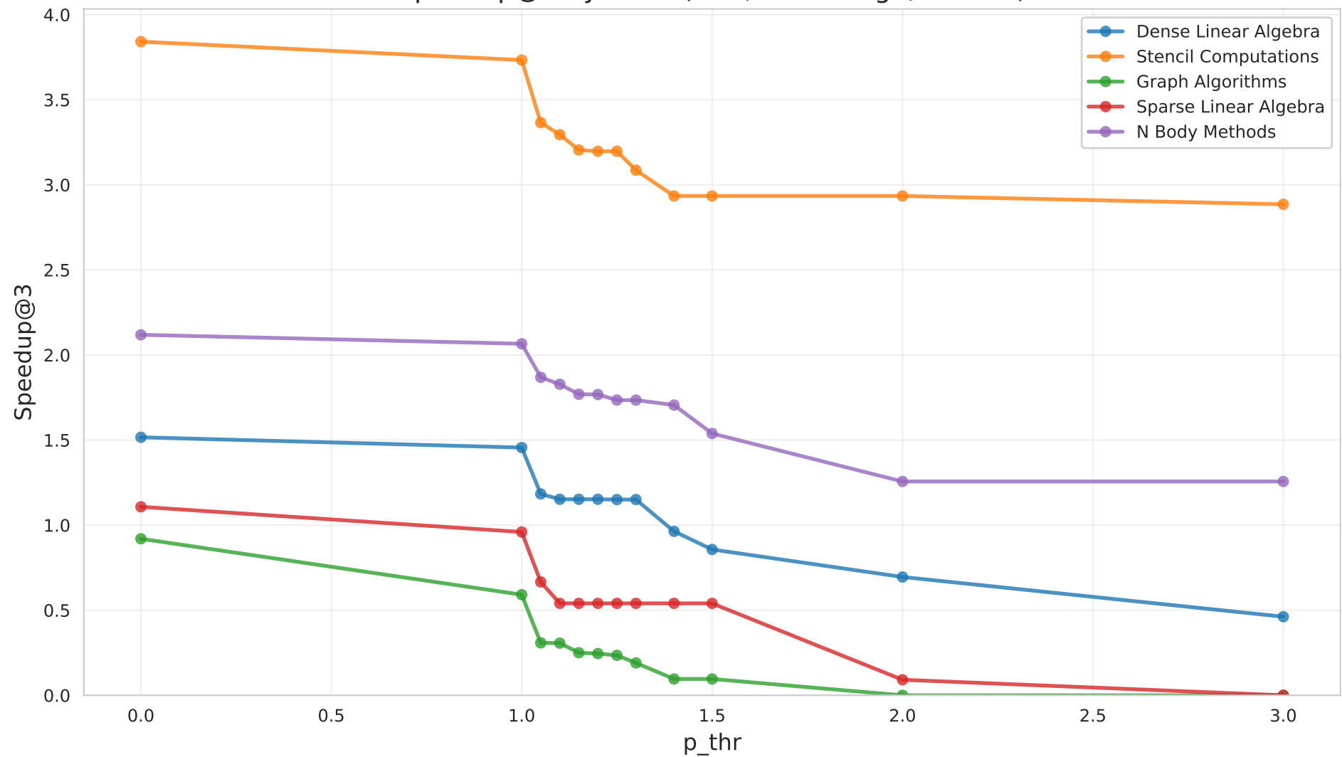
Speedup@3 by Motif (EX1, extra-large, Claude)
