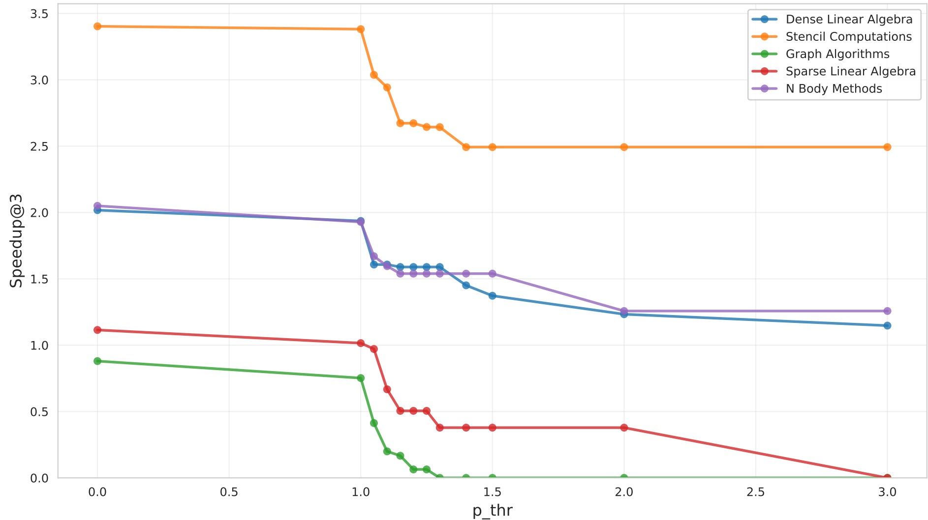
Speedup@3 by Motif (EX1, large, Claude)
