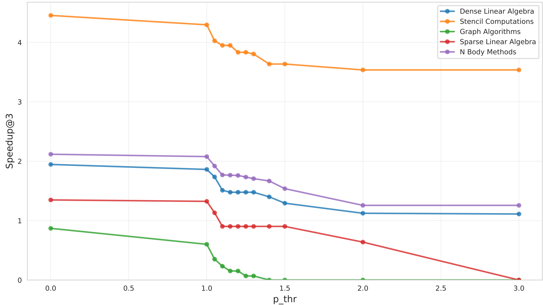
Speedup@3 by Motif (EX1, medium, Claude)
