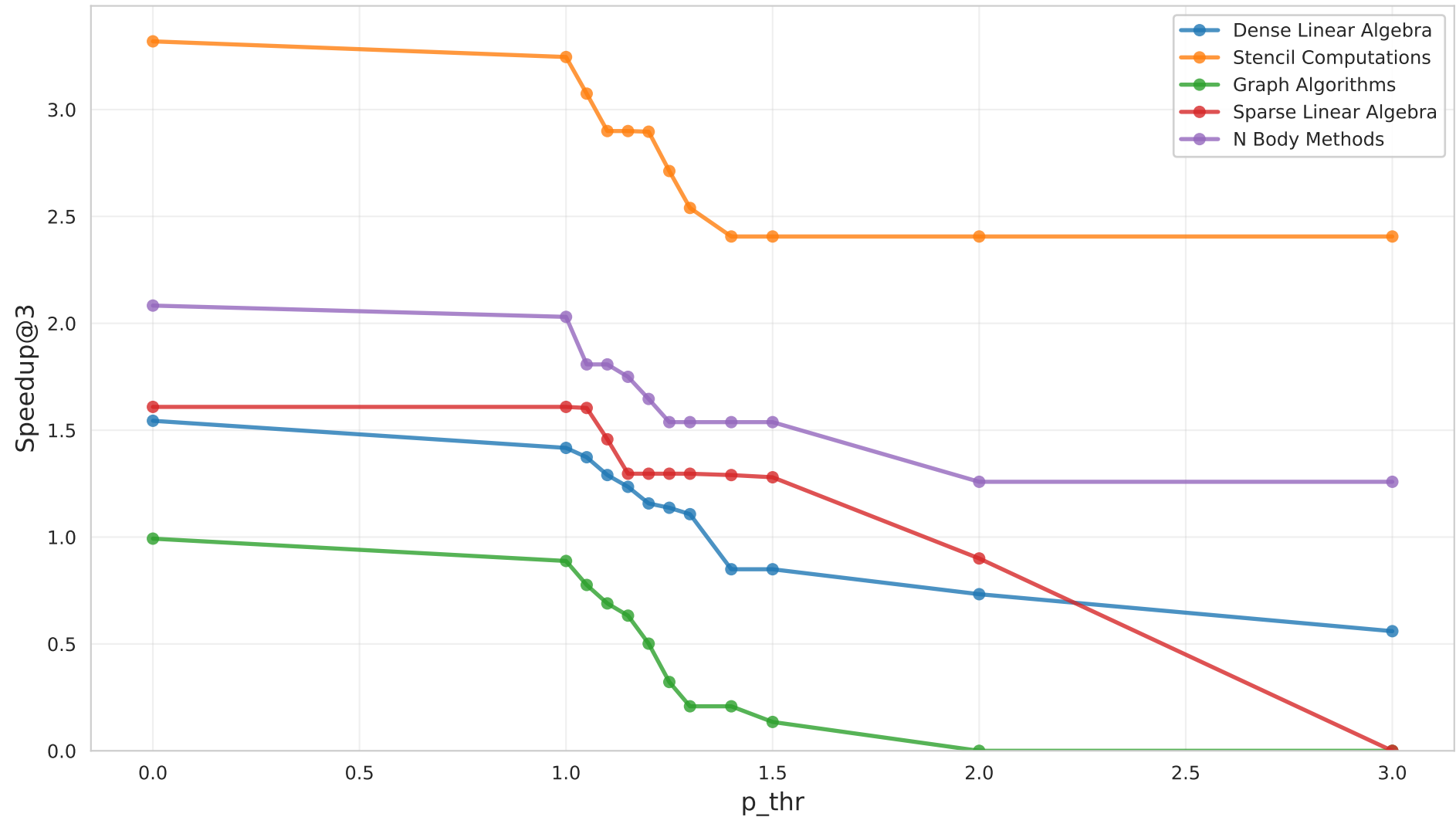
Speedup@3 by Motif (EX1, mini, Claude)
