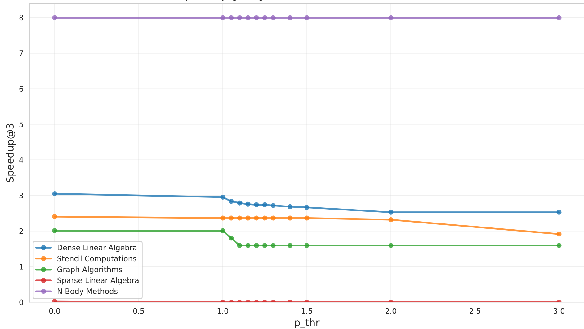
Speedup@3 by Motif (EX2, medium, Claude)
