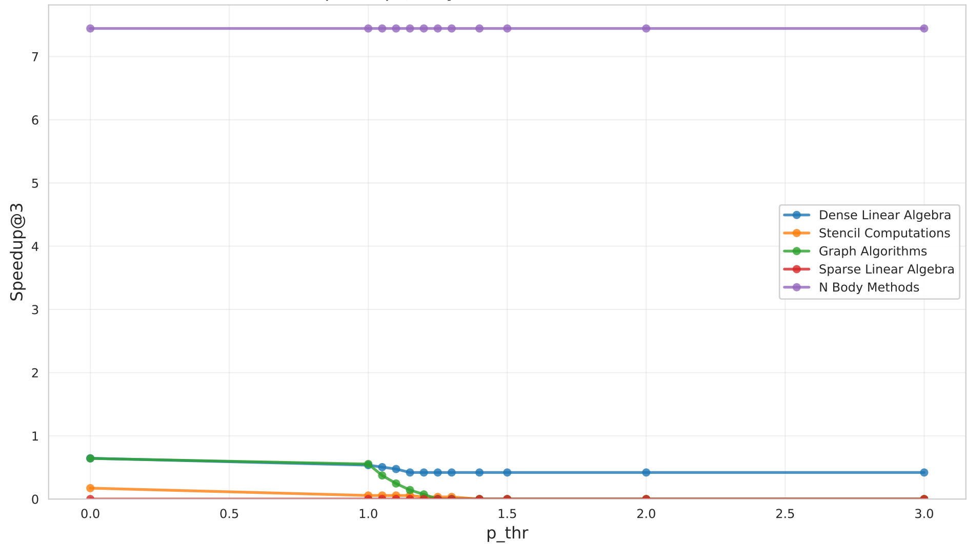
Speedup@3 by Motif (EX2, mini, Claude)
