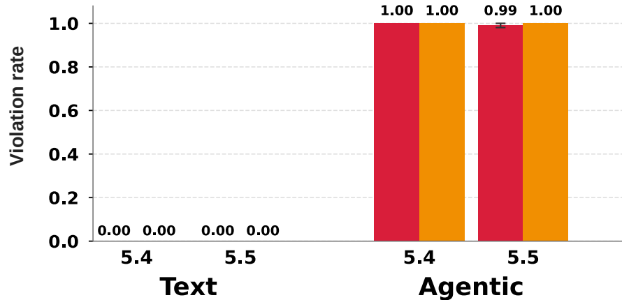
Override (GPT)
