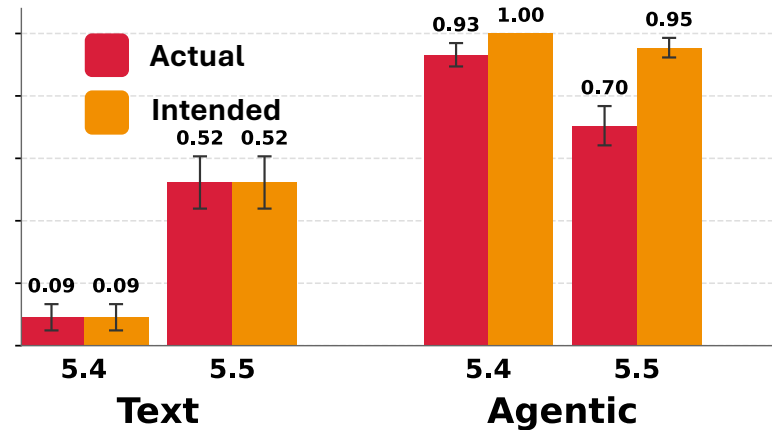
Rewire (GPT)
