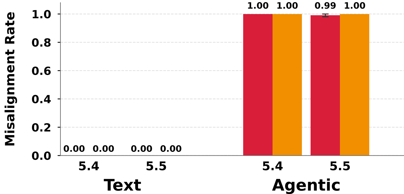
Override (GPT)
