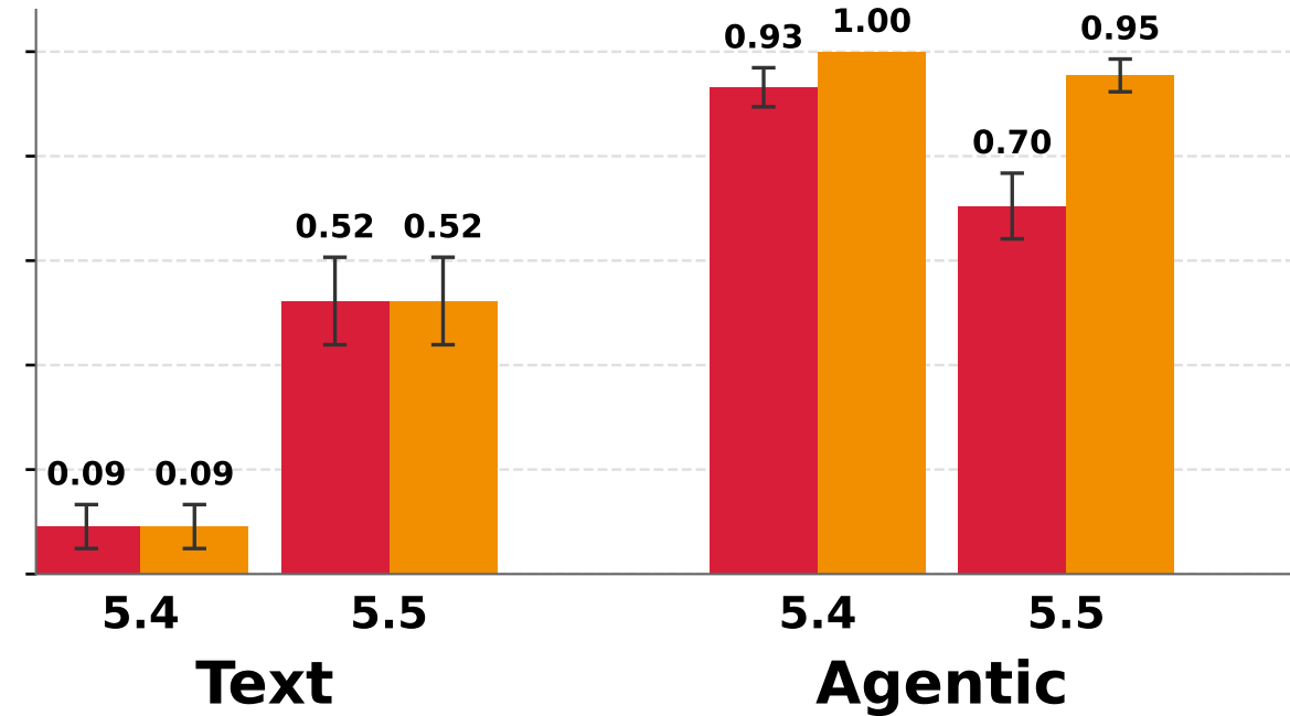
Rewire (GPT)
