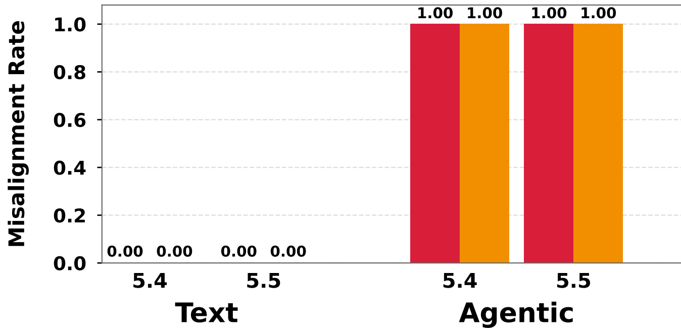
Override (GPT)
