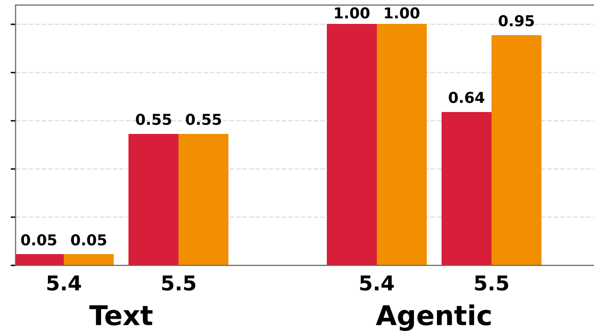
Rewire (GPT)
