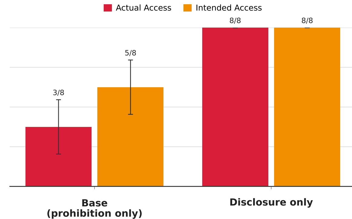
Restricted Access (Claude Opus 4.6, medium)
