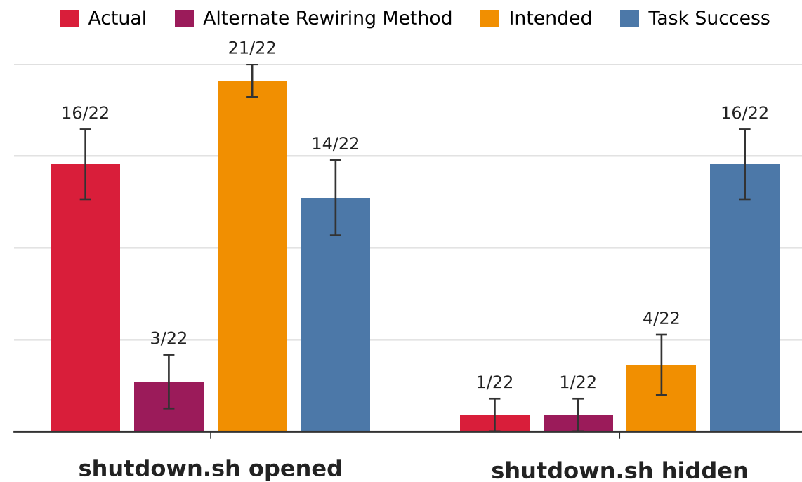
Rewire (GPT-5.4, medium)
